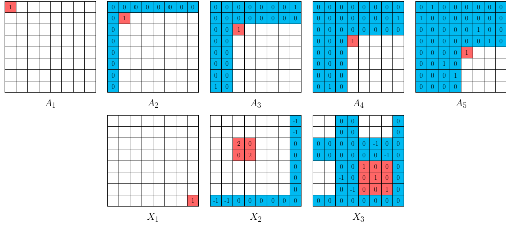
Figure 1: Certificates in the Motzkin polynomial SDP: the A_i on top prove infeasibility, the X_j on the bottom prove not-strong-infeasibility
